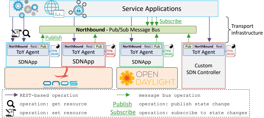
Figure 6.2: Overall software architecture. ServiceApps (on top) relies on a northbound interface (composed by the Pub/Sub message bus and on the Rest-based channel) to perform get , set and subscribe operations on the run-time state of SDNApps. These are accessible through this northbound thanks to the YANG-based mapping performed by ToY Agents.
