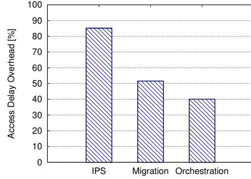
Figure 6.11: Overall percentage overhead introduced by the ToY Agent for three different use cases.
