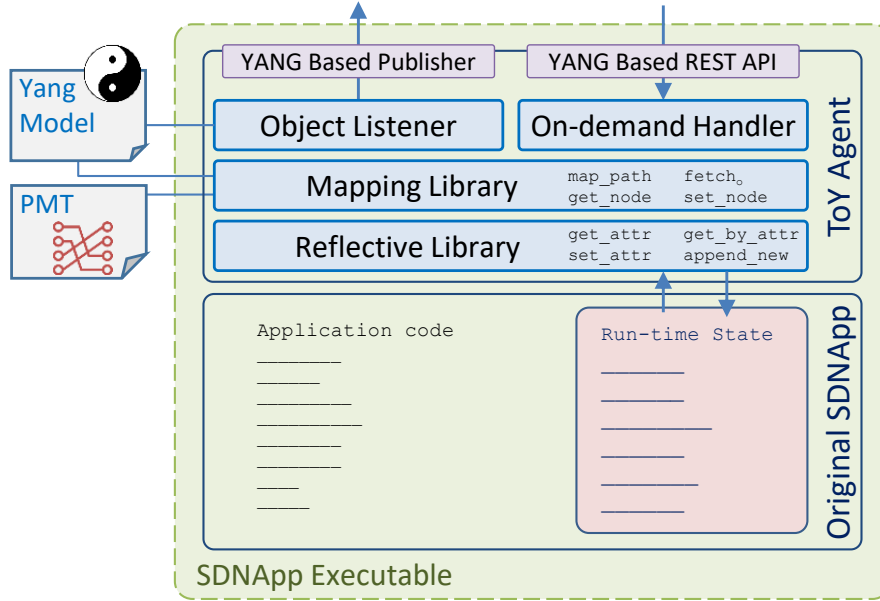
Figure 6.6: Architecture of the ToY Agent.
