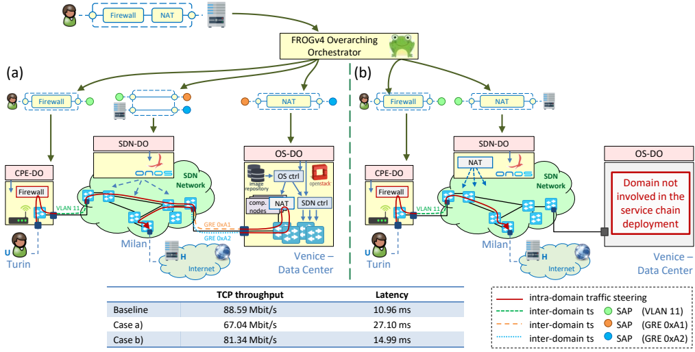
Figure 2.6: Deployment of a service graph in two different scenarios. In case (b), the SDN-DO provides the capability of running a NAT (as SDN application), thus the Overarching Orchestrator opts for better optimization. Performances are compared at the bottom.
