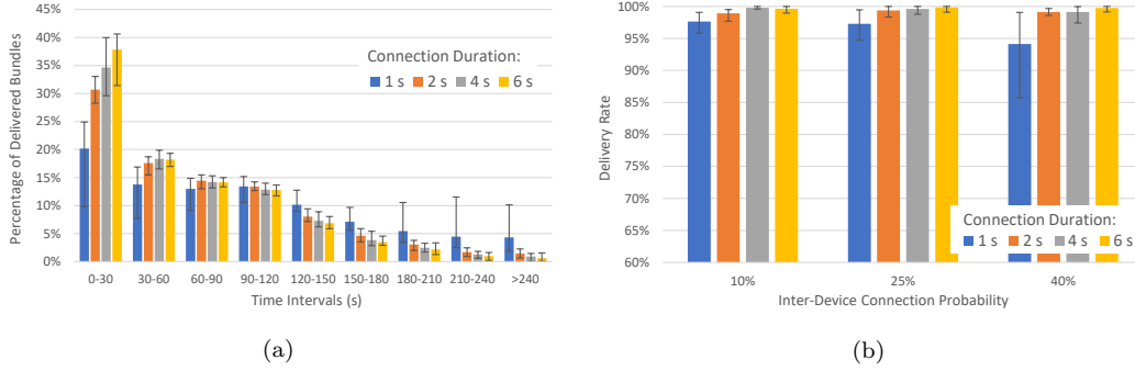
Figure 7.10: (a) Distribution over time of delivered bundles, for different connection time intervals. (b) Bundle delivery ratio varying the probability of inter-device connections, comparing different connection time intervals (1, 2, 4 and 6 seconds). All values refer only to bundles already expired at the end of the run.
