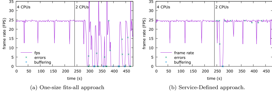
Figure 4.4: Frame rate over time for a video streaming application in a resource constrained situation. A Service-Defined Orchestrator may effectively mitigate the QoE deterioration being able to explore alternative solutions.
