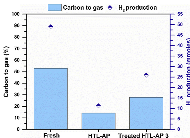
Fig. 11. APR of glycolic acid with different catalysts. Reaction conditions: Liquid phase amount 75 g, 0.9 wt.% C glycolic acid, reaction temperature 270 °C, reaction time 2 h.
