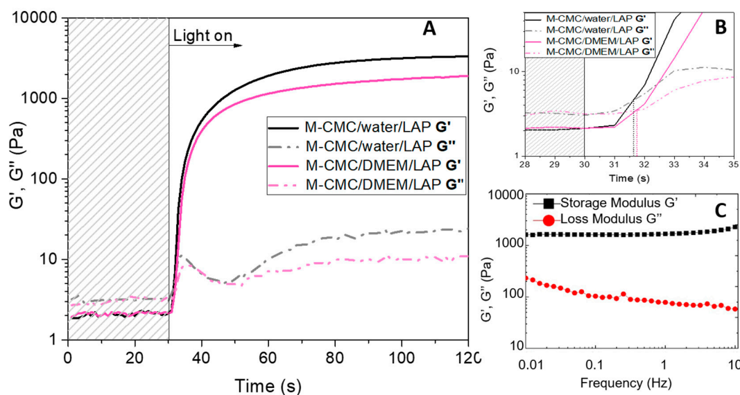
Figure 2. (A) Photorheology of methacrylated carboxymethyl cellulose (M-CMC) 20 mg/mL (2 wt% lithium phenyl-2,4,6-trimethylbenzoylphosphine (LAP)) solubilized in water (black) or in culture medium (pink). (B) Gel point. Film thickness 300 m. (C) Frequency sweep. Strain rate 1% and oscillation frequency from 0.01 to 10 Hz.
