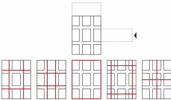
Figure 12. Position of the section planes. Drawing: F. Natta
