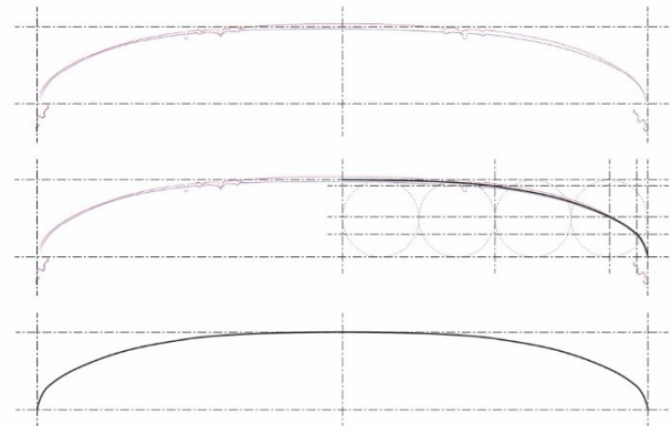
Figure 13. Tracing method for directrices and comparison with the section of point cloud (red). Drawing: F. Natta
