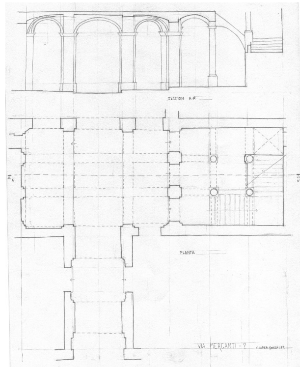
Figure 6. Previous preparation drawing. Section and plan of the atrium. Drawing: M. C. López González
