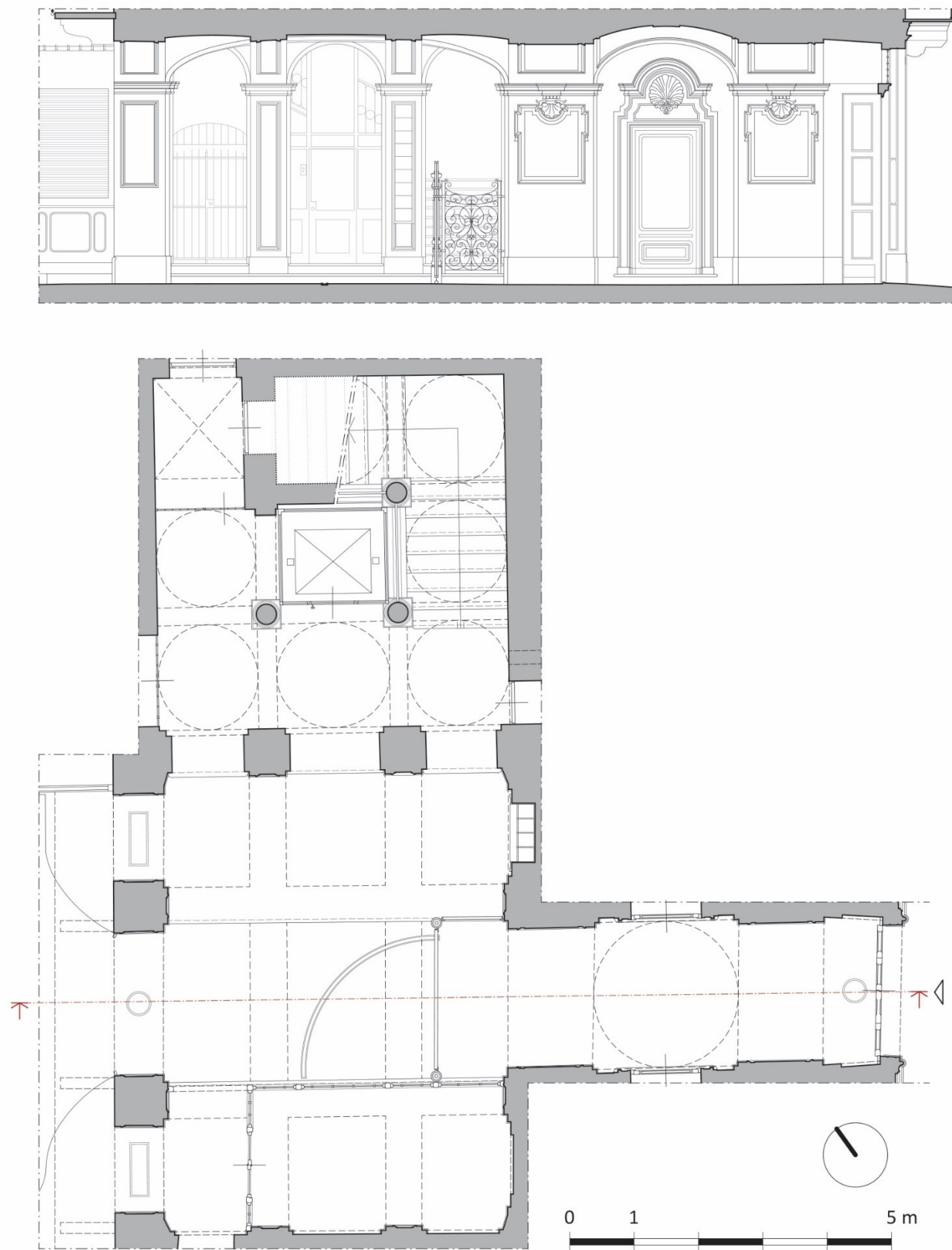
Figure 11. Survey drawings of the atrium in Via dei Mercanti 2. Drawing: F. Natta
