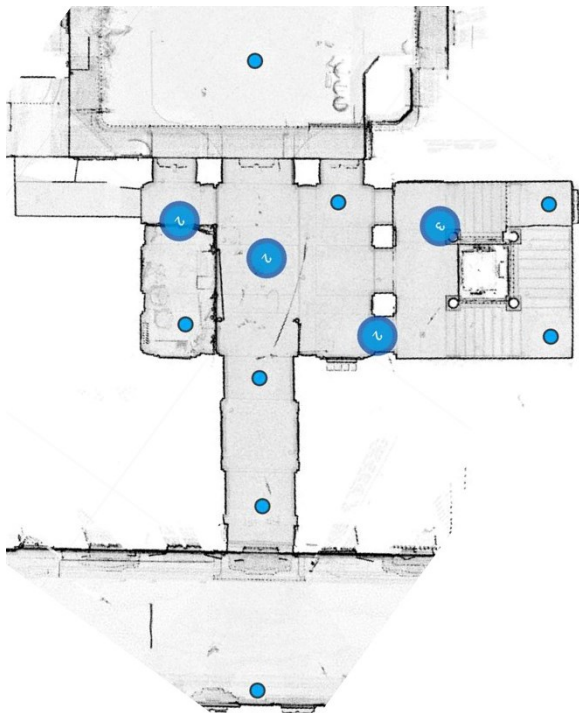
Figure 9. Location of scan points. Scanning: M. C. López González. Processing: F. Natta
