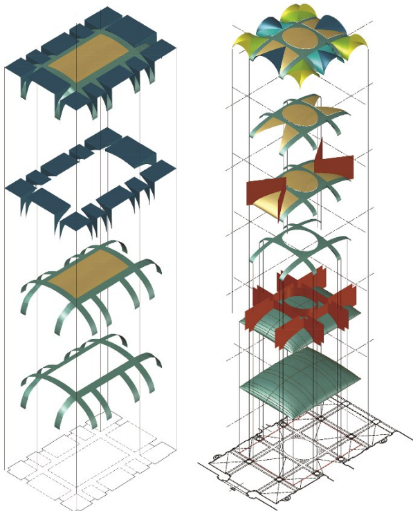
Figure 5. Decomposition method for banded vaults with independent arches (left) and with arches belonging to the main surface (right). Modelling: R. Spallone, M. Vitali
