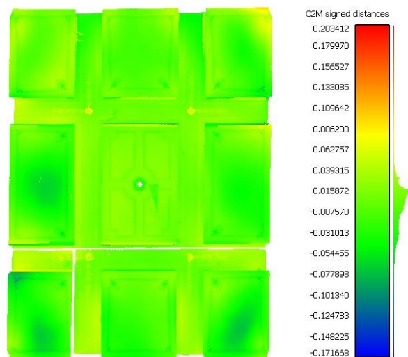
Figure 16. Distances between point cloud and ideal model. Processing: F. Natta
