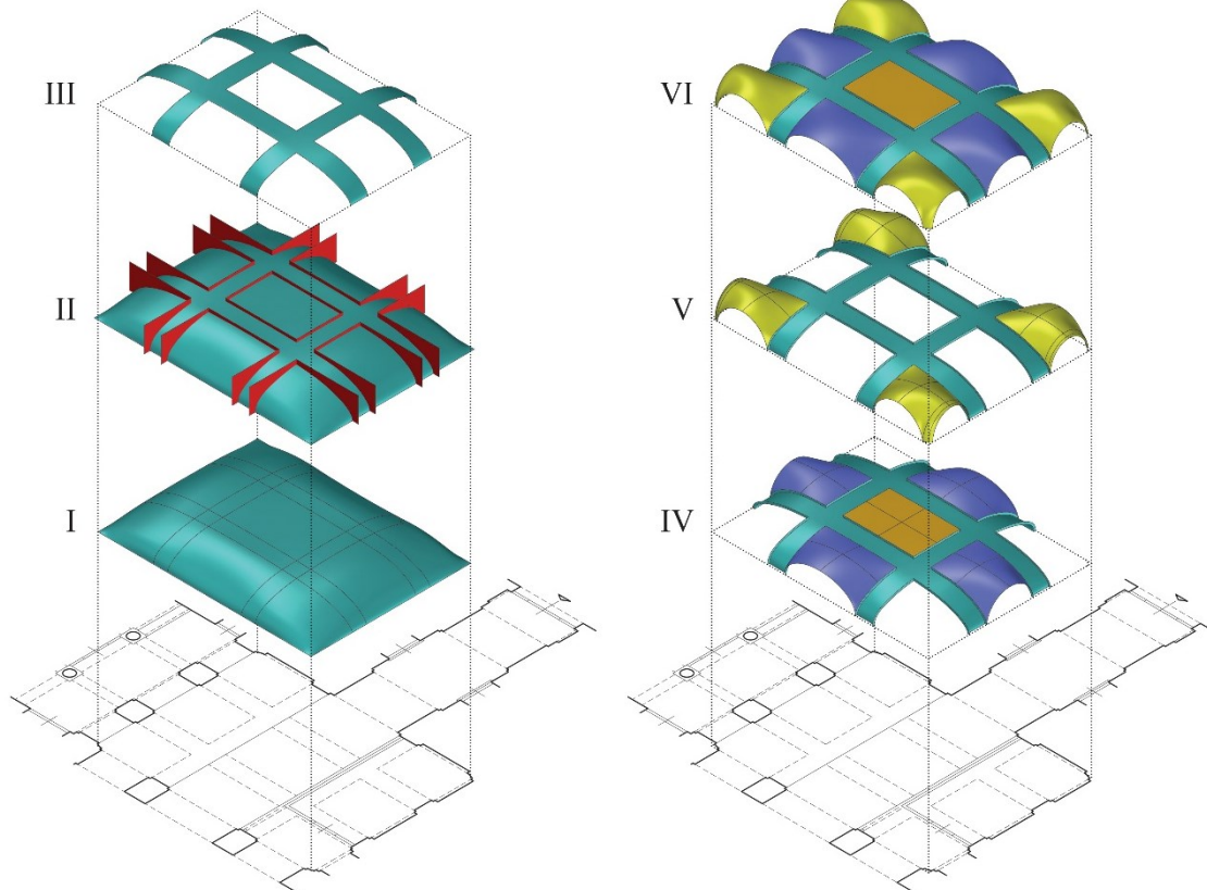
Figure 14. Decomposition of the 3D model of the vault design shape. Modelling: F. Natta
