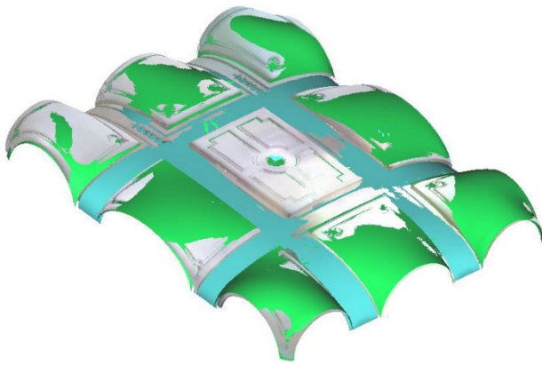
Figure 15. Superimposition of point cloud and ideal design model. Processing: F. Natta
