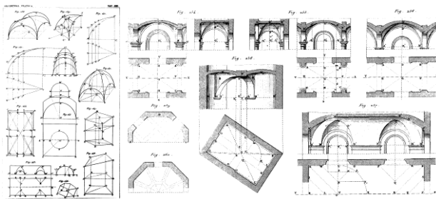
Figure 3. “A fascioni” vaults on a rectangular plan, geometric scheme (left) and architectural representation in orthographic projections (right). Sources: Curioni, 1868, Plate XIII; Curioni, 1865, Plate XXV
