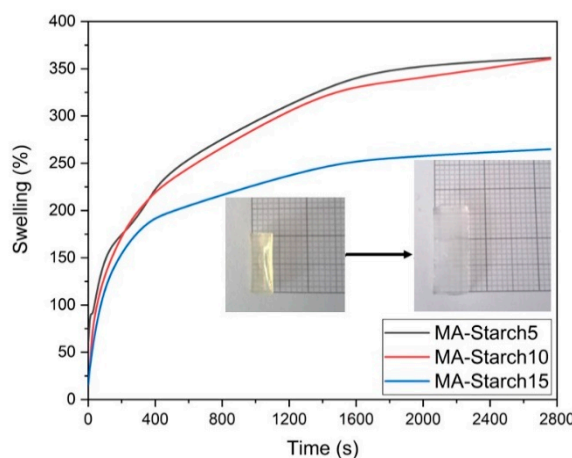
Figure 5. Swelling behavior of the three MA-Starch derived hydrogel formulations.
