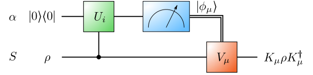
FIG. 3. Strictly incoherent operations on system S constructed by an incoherent unitary interaction with an ancilla \alpha . An operation is split into a controlled unitary \sum_i |i\rangle\langle i|_S \otimes (U_i)_\alpha followed by a measurement on the ancilla in a basis |\phi_\mu\rangle and an incoherent unitary V_\mu on the system conditioned on the measurement outcome \mu .
