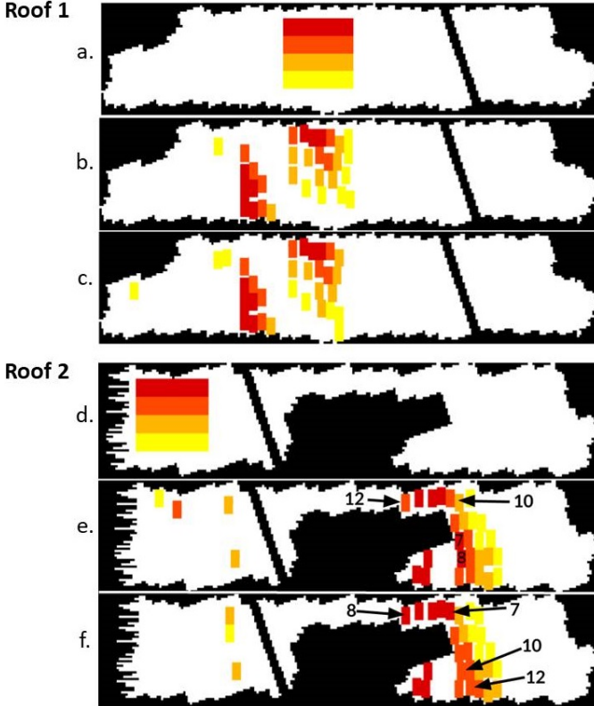
Fig. 4. Possible configuration for N=32 for roof 1 ( a-c ) and roof 2 ( d-f ): traditional “compact” placement ( a,d ), placement generated by [22] ( b,e ), proposed algorithm ( c,f ). Rectangles are PV modules, rectangles of the same color are PV modules connected in series.
