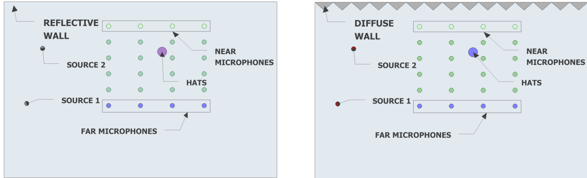
Figure 2. Scheme of ESPRO's (IRCAM) coated wall with case C conditions: reflective (left) and diffusive (right). Boxed: 4 microphone positions near and far away the reflective and diffusive wall.
