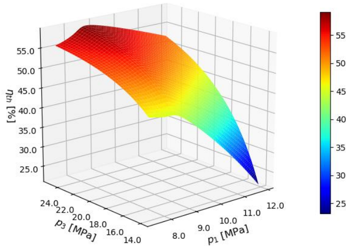
Figure 17 Thermodynamic efficiency of the REG CO_2 cycle.
