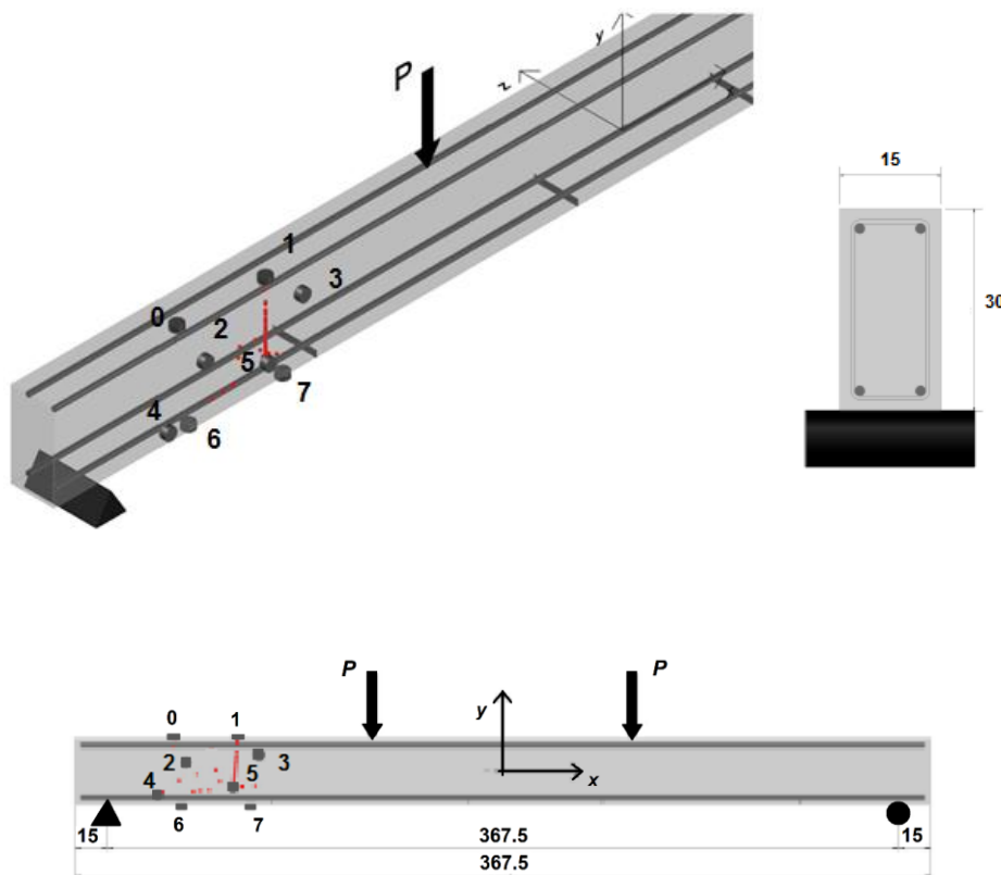
Figure 1. Specimen geometry and acoustic emission (AE) sensor locations. The eight AE sensors are numbered from 0 to 7. Dimensions are in cm.
