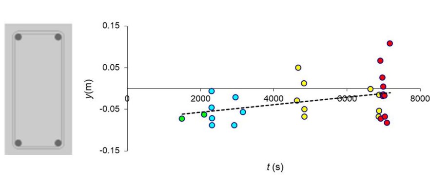
Figure 9. Height of localized AE events for different loading stages. Adopted reference system ( x , y , z ) as in Figure 1. Green color refers to load stages #1–#4, blue to #5 and #6, yellow to #7 and #8, and red to #9.
