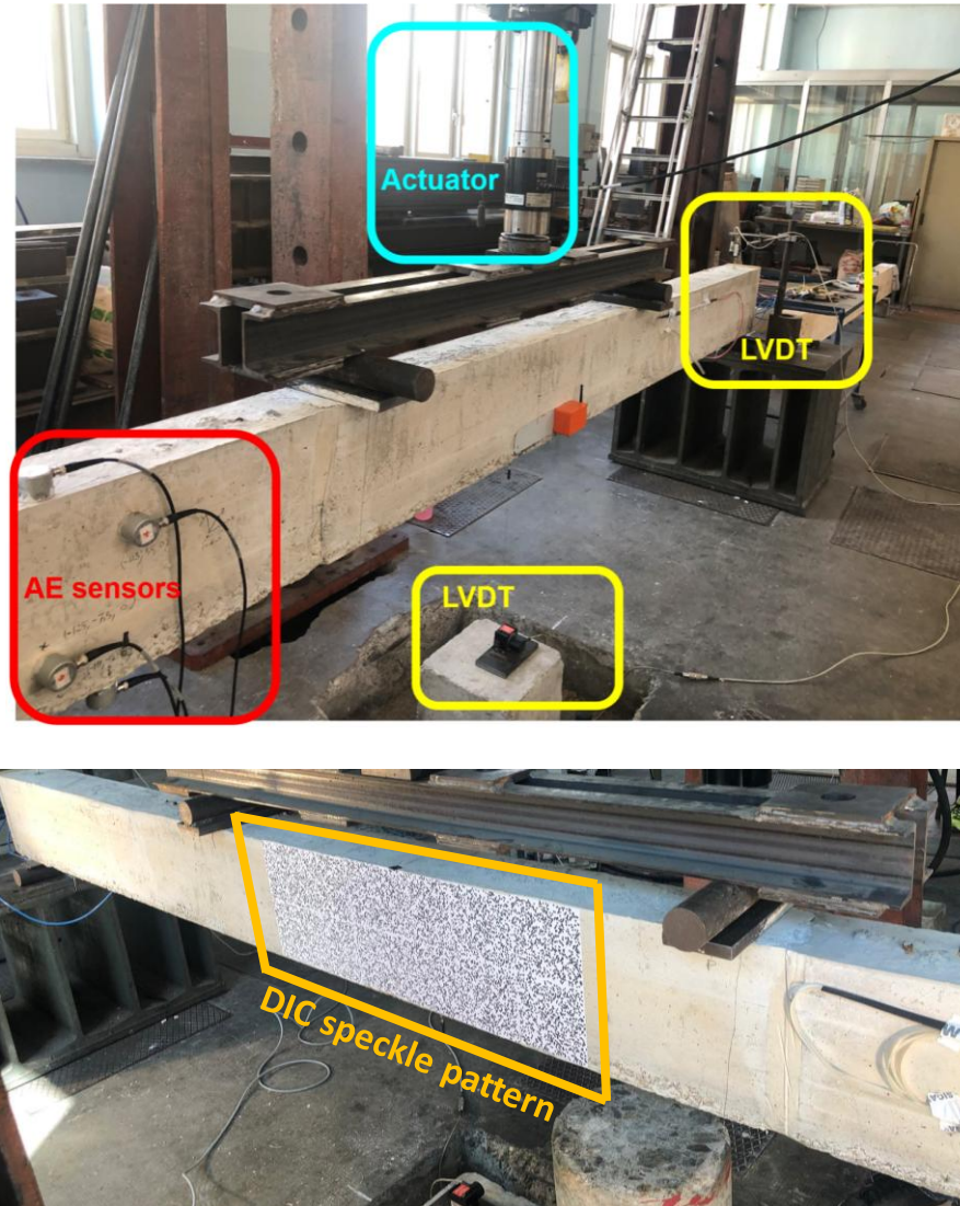
Figure 2. Front (top) and back (bottom) sides of the test setup showing the servo hydraulic actuator, the linear variable differential transformer (LVDT) sensors, the location of some AE sensors, and the speckle pattern on the central beam surface for digital image correlation (DIC) applications.
