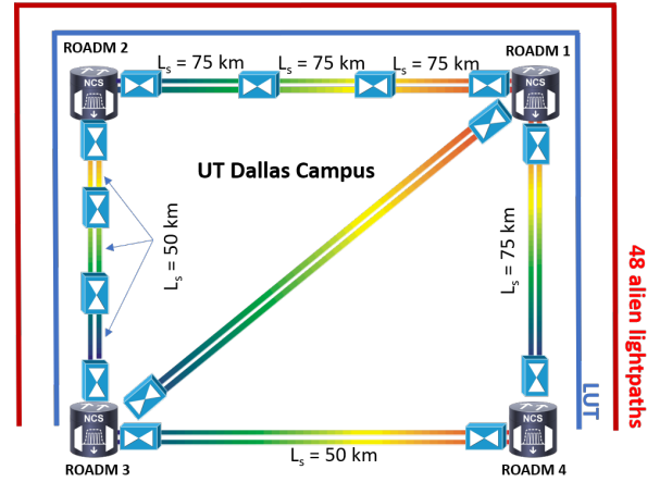
Fig. 2. PRONet topology.
