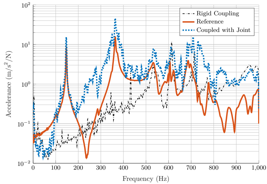
Fig. 11: The on-board validation of the joint. The solid validation line is a measured FRF of the full-system. This FRF (at the DoF marked with squares in Fig. 7c) has not been used to identify the joint. The blue dotted line indicates the coupled results (with the joint identified by the SEMM procedure). The dash-dotted black line is the would-be rigid coupling (without joint). The coupled results are not in good agreement with the full-system reference FRF but outperform the rigid coupling.
