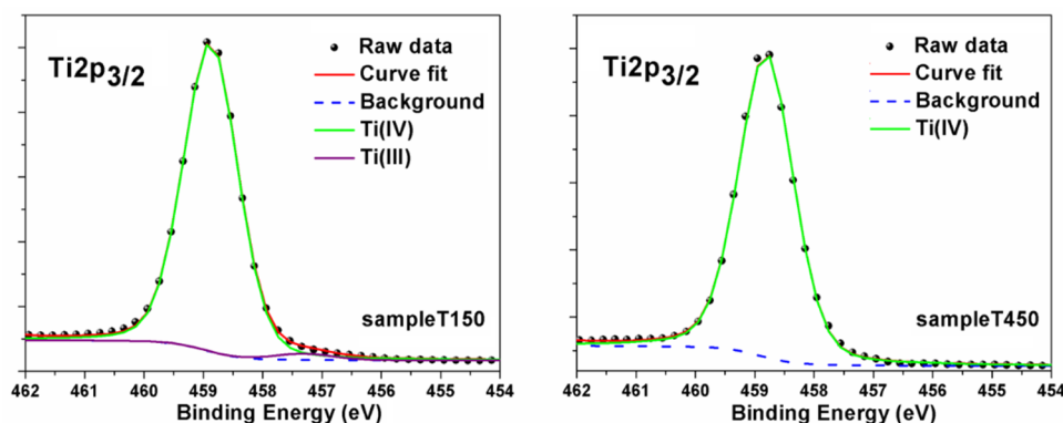
Figure 3. Ti 2p 3/2 X-ray photoelectron spectroscopy (XPS) peaks for T150 (left) and T450 (right) samples. Curve fitting results have been reported, by showing raw data (scatter black dots), curve fit (red line), Shirley background function (blue dash line), and Ti components (green line for Ti(IV) and purple line for Ti(III)).
