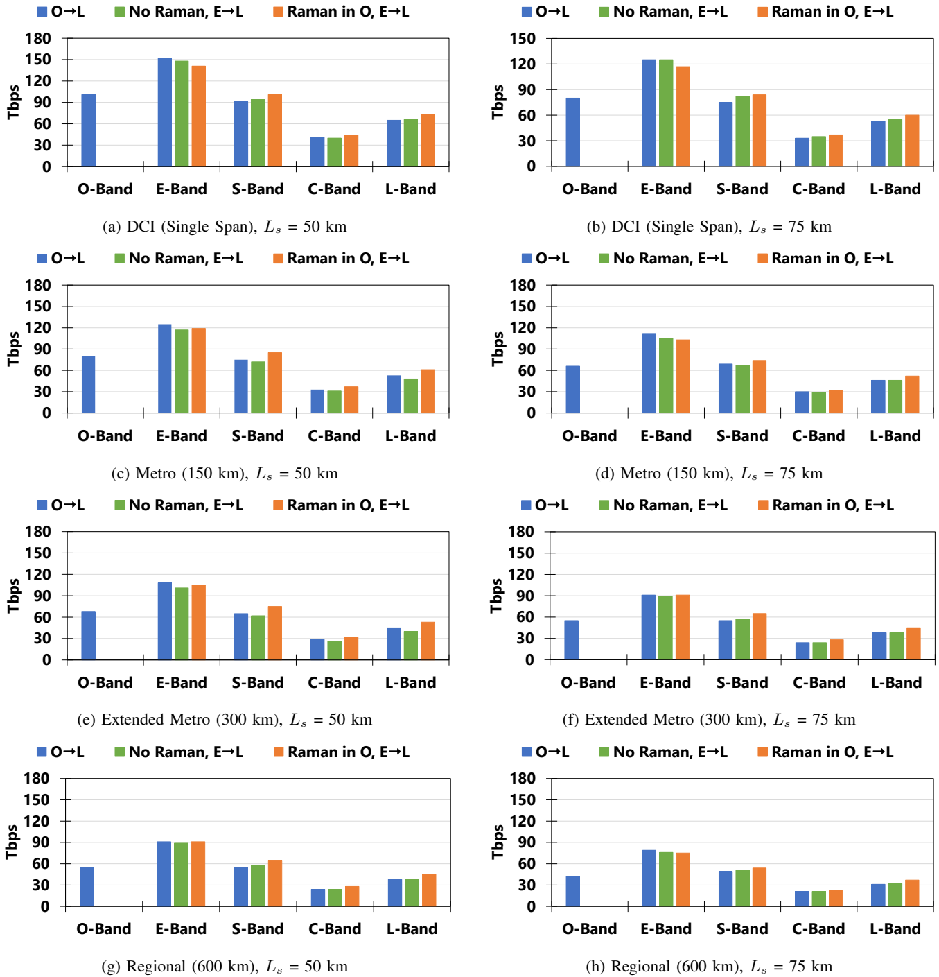
Fig. 10: Maximum capacity per transmission band. Each row refers to a different reach: DCI (75 km) the first, metro (150 km) the second, extended metro (300 km) the third and regional (600 km) the last one. Left-hand side: 50 km spans; and right-hand side: 75 km spans.
