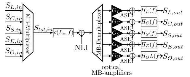
Fig. 6: Equivalent block diagram of a span.
