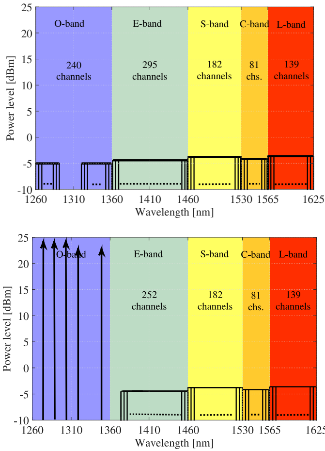
Fig. 5: Considered system configurations: a) Full MBT; b) O-band off, Raman in O-band, E → L-band.
