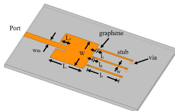
Fig 1. Geometrical representation of the graphene antenna.
