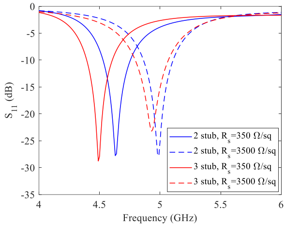
Fig. 3. Comparison of the return loss of the two stub antenna with the three stub antenna.
