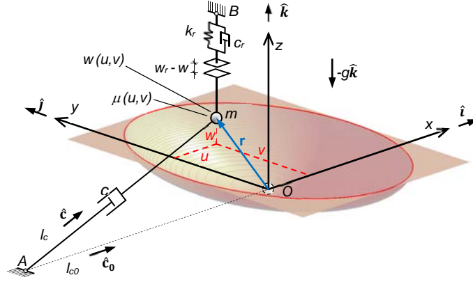
Figure 3. Axonometric scheme of the BTMD model.
