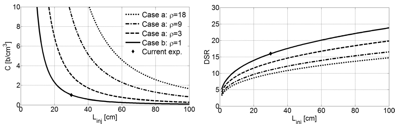
Fig. 2 Concentration ( left ) and DSR ( right ) as function of the characteristic length of the injector and of the contraction ratio. Equation (7) is used to retrieve C . DSR was computed using Eq. (6) where L is replaced by the relation expressed in Eq. (8) ( \dot{N} = 8 \times 10^6 , U_\infty = 8.5 m/s)
