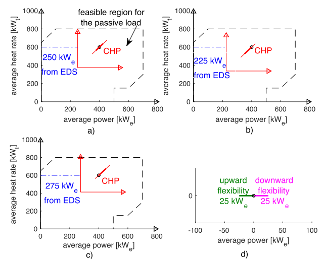
Fig. 22. Dynamic flexibility region reduced by time-dependent limits. (a) Reference case for the usage of the CHP. (b) Maximum reduction in the average power taken from the EDS. (c) Maximum increase of the average power taken from the EDS. (d) Upward and downward dynamic flexibility.
