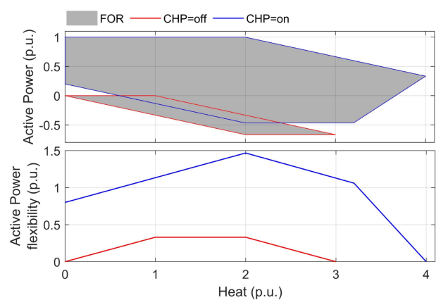
Fig. 15. FOR in the (top) H-P plane and (bottom) electrical flexibility of test system 3 with CHP ON/OFF.
