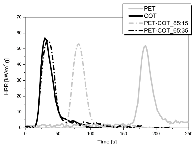
Figure 4. Heat Release Rate (HRR) curves of PET, COT, PET-COT_85:15 PET-COT_65:35 fabrics. Data obtained by cone calorimetry under 35 \text{ kW/m}^2 .
