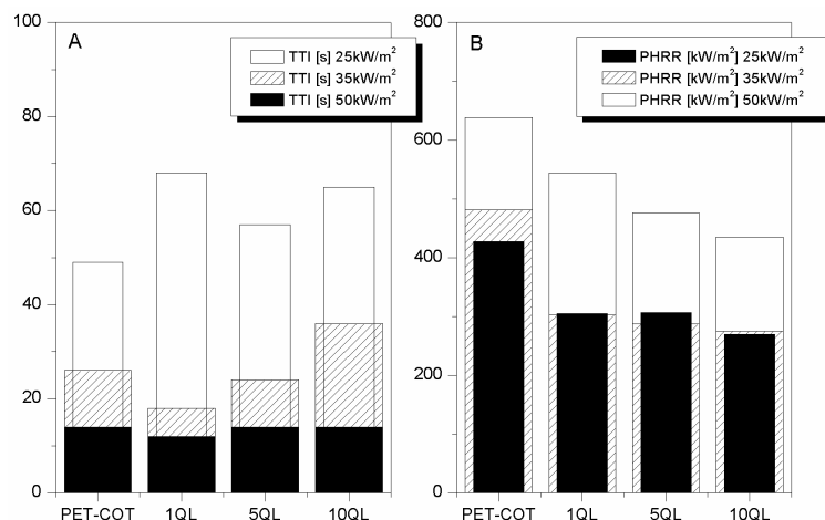
Figure 12. TTI (A) and PHRR (B) values of PET-COT fabrics treated with 1, 5 and 10 QL at 25, 35, and 50 kW/m² [29].
