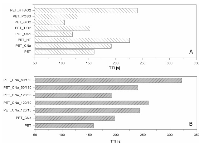
Figure 2. TTI values of nanoparticle (NP)-treated polyethylene terephthalate (PET) fabrics (A) and treated initially by plasma and then with CNa suspension (B) [33,35]. Data obtained by cone calorimetry at 35 kW/m 2 .
