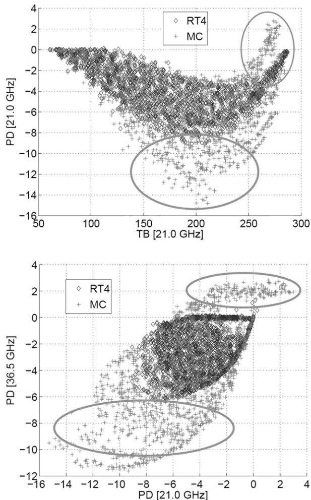
FIG. 9. Scatterplots between SP RT4 and Monte Carlo computations to highlight “3D scattering effects.” The geometry of the simulations is the one illustrated in Fig. 6 with an elevation angle of 30°, L_x = L_y = 4 km and P_x = (-3.5:1.0:3.5) km. About 3000 profiles with freezing levels ranging from 2 to 4 km are considered in this example: (top) PD vs T_B and (bottom) PD vs PD.
