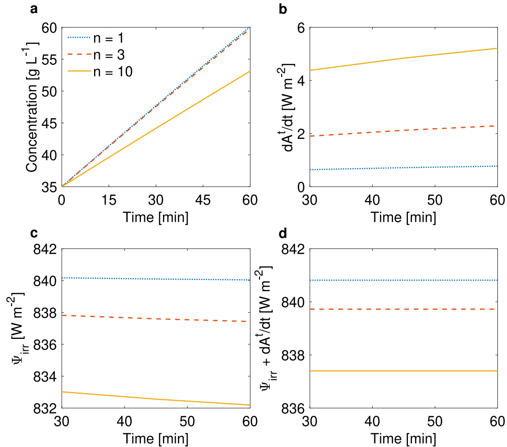
Fig. 4. Transient exergy analysis of the improved version of the device for different number of distillation stages ( n ). (a) Salt concentration of the solution in the evaporators, (b) exergy storage due to salt accumulation, (c) irreversibility production and (d) sum of the exergy storage and irreversibility production. In detail, three different configurations are considered: dotted blue, dashed red and yellow lines represent the 1-, 3- and 10-stage devices, respectively.
