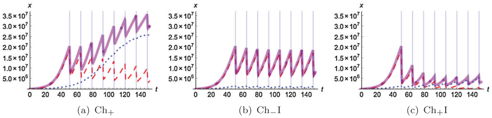
Figure 1. Time courses of x_1 (red dashed line) x_2 (blue dotted line) and total cancer population x (continuous purple line), in the COE case. The cyan vertical lines correspond to the administration of medication during the pulsed therapy. (a): Standard chemotherapy dose ( Ch_+ ). (b): Combination of low chemotherapy dose and immunotherapy ( Ch_-I ). (c): Combination of standard chemotherapy dose and immunotherapy ( Ch_+I ).
