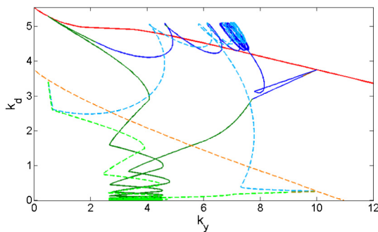
Fig. 10. Lower costs of investment in defense capital ( \theta_1 = 0.25 , dashed lines) shift the Skiba curve (orange dashed line instead of red solid line) and enlarge the region where economies become a rich economy compared to the base case ( \theta_1 = 0.5 , solid lines). k_y and k_d are the physical capital and the defense capital, respectively. (For interpretation of the references to color in this figure legend, the reader is referred to the web version of this article.)
