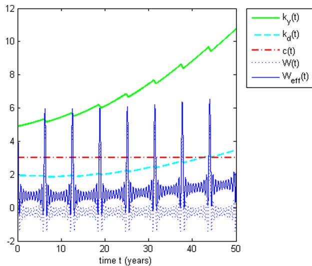
Fig. 6. Simulation run where the initial values k_d(t_0) = 2 and k_y(t_0) = 5 are enough to enable economic growth if the investment in defense capital is only 25% of the total investment.
