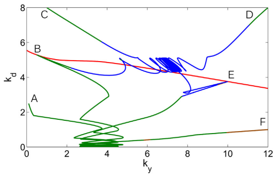
Fig. 9. Different initial conditions (points A–F) in several economies induce to different long-term behavior. The red line (Skiba curve) separates the initial values leading to a rich or to a poor economy. k_y and k_d are the physical capital and the defense capital, respectively.
