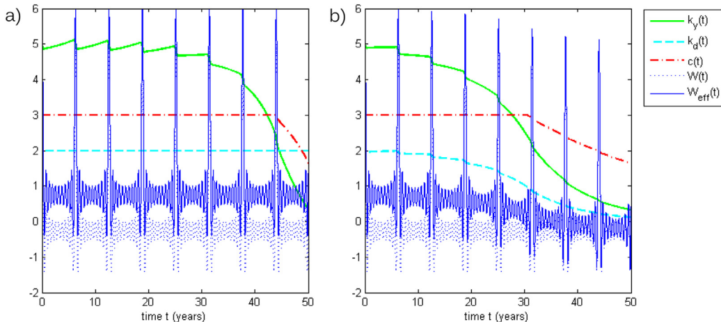
Fig. 5. Simulation run of the physical capital k_y(t) , the defense capital k_d(t) , the consumption c(t) , the exogenous water level W(t) and the endogenous effective water level W_{eff}(t) . a) Constant k_d = 2 with k_y(t_0) = 5 and b) proportional investments with k_d(t_0) = 2 and k_y(t_0) = 5 run into economic disaster.
