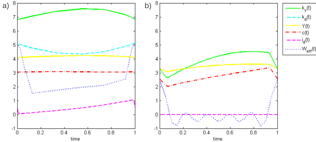
Fig. 7. One limit cycle (in normalized time) of the long-term behavior of a a) rich economy, b) poor economy showing the time series of the physical capital k_y(t) , the defense capital k_d(t) , the economic output Y(t) , the consumption c(t) , the investment in defense capital i_d(t) and the exogenous effective water level W_{eff}(t) = W(t) + \zeta_d k_d(t) .
