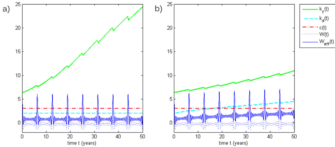
Fig. 4. Simulation run of the physical capital k_y(t) , the defense capital k_d(t) , the consumption c(t) , the exogenous water level W(t) and the endogenous effective water level W_{eff}(t) . a) Constant k_d = 2 with k_y(t_0) = 6.5 and b) proportional investments with k_d(t_0) = 2 and k_y(t_0) = 6.5 lead to economic growth. The unit of k_y and c(t) is [$], all the other variables are given in [m].
