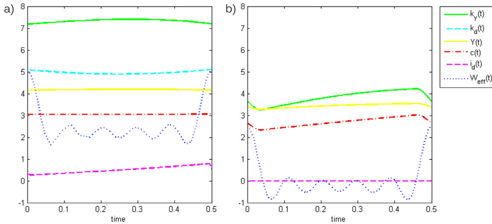
Fig. 11. One limit cycle in case of a higher frequency of floods and therefore time period [0,0.5] for a) a rich economy, b) a poor economy. Parameters as in base case of Table 2, but \kappa_m = 2 . Note, since we plot only one period and the frequency of the periods changed, the time interval is now only [0, 0.5].
