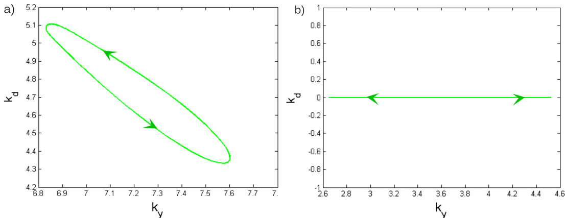
Fig. 8. The state dynamics of the a) rich economy, b) poor economy.
