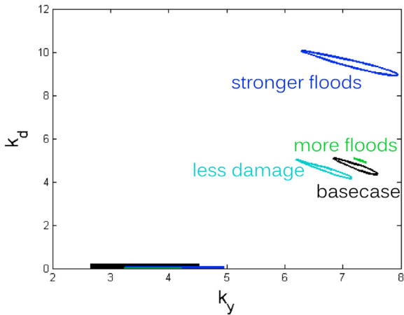
Fig. 15. Long-term state dynamics for the cases of Figs. 7–13. (For interpretation of the references to color in this figure, the reader is referred to the web version of this article.)
