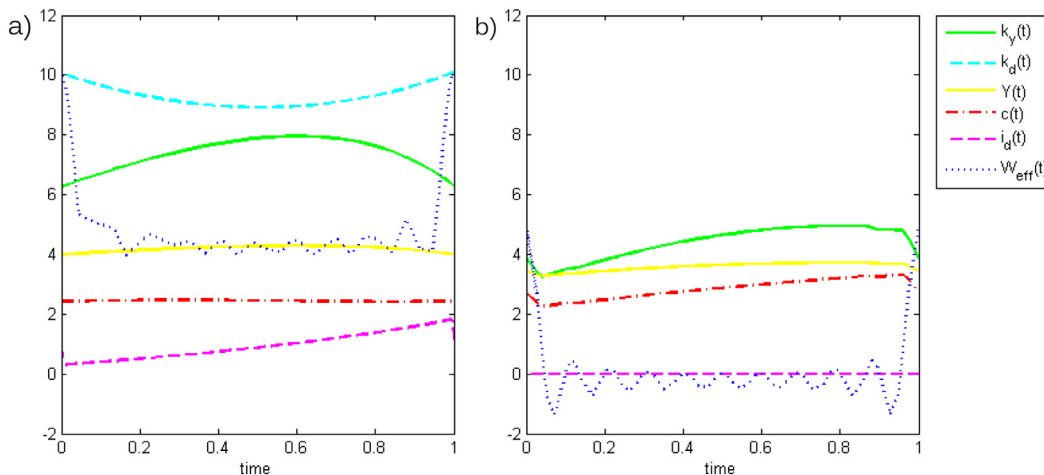
Fig. 12. One limit cycle in case of bigger floods for a) a rich economy, b) a poor economy. Parameters as in base case of Table 2, but \kappa_s = 10 .
