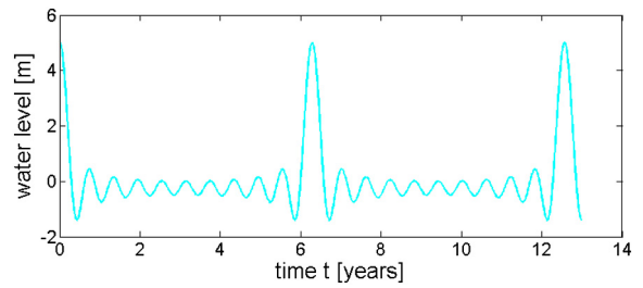
Fig. 3. The periodic water level function gives quite frequent flood events. In brackets we display the units for the time and the water level itself.
