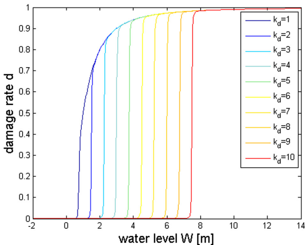
Fig. 2. Form of the damage rate as a function of the water level W(t) for various levels of the defense capital k_d(t) and for \xi_d = 0.5 . Both the water level and the defense capital are given in meters.
