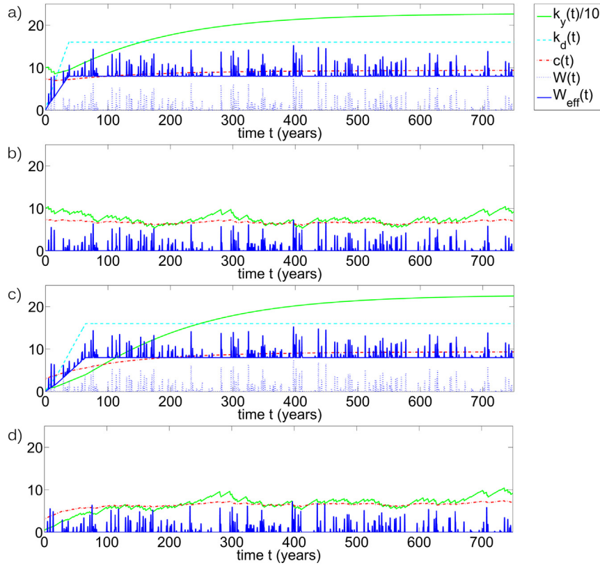
Fig. 14. Simulation runs of the physical capital k_y(t) , the defense capital k_d(t) , the consumption c(t) , the exogenous water level W(t) and the endogenous effective water level W_{eff}(t) . The unit of k_y(t) and c(t) is [$], all the other variables are given in [m]. a) and c) show the scenario of the rich economy and b) and d) the poor economy. The initial conditions for a) and b) are k_y(t_0) = 100 and k_d(t_0) = 0 , for c) and d) k_y(t_0) = 5 and k_d(t_0) = 0 .
