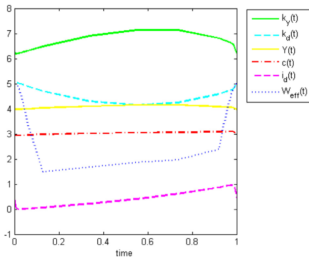
Fig. 13. One limit cycle in case of a more robust flood defense capital. Parameters as in base case of Table 2, but \kappa_d = 0.1 . Note, due to numerical discretization of the solution W_{eff} is displayed different, but has the same oscillating behavior as in the other figures.
