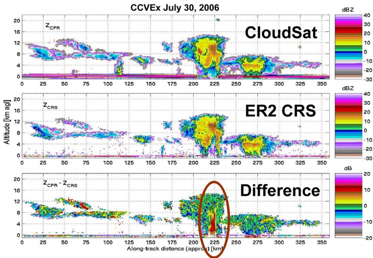
Figure 1. Evidence of multiple-scattering effects from the airborne CloudSat/CALIPSO Validation Experiment (CCVEx). (top) CloudSat radar reflectivity in \text{dBZ} ; (middle) ER2-CRS radar reflectivity in \text{dBZ} under flying the CloudSat ground track; and (bottom) difference between the CPR and the CRS reflectivities in decibels. This image, courtesy of S. Tanelli (Jet Propulsion Laboratory, California Institute of Technology), was generated using CRS preliminary calibration data courtesy of G. Heymsfield (NASA/GSFC) and L. Li (GEST). Relative calibration between CPR and CRS has been corrected since, and this image should be regarded as calibrated within 3 dB. The MS signature due to the different footprint sizes is evident well beyond this calibration uncertainty.
