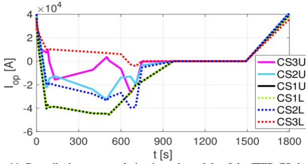
Fig. 11. Prescribed current evolution in each module of the ITER CS during the standard 15 MA plasma pulse.
