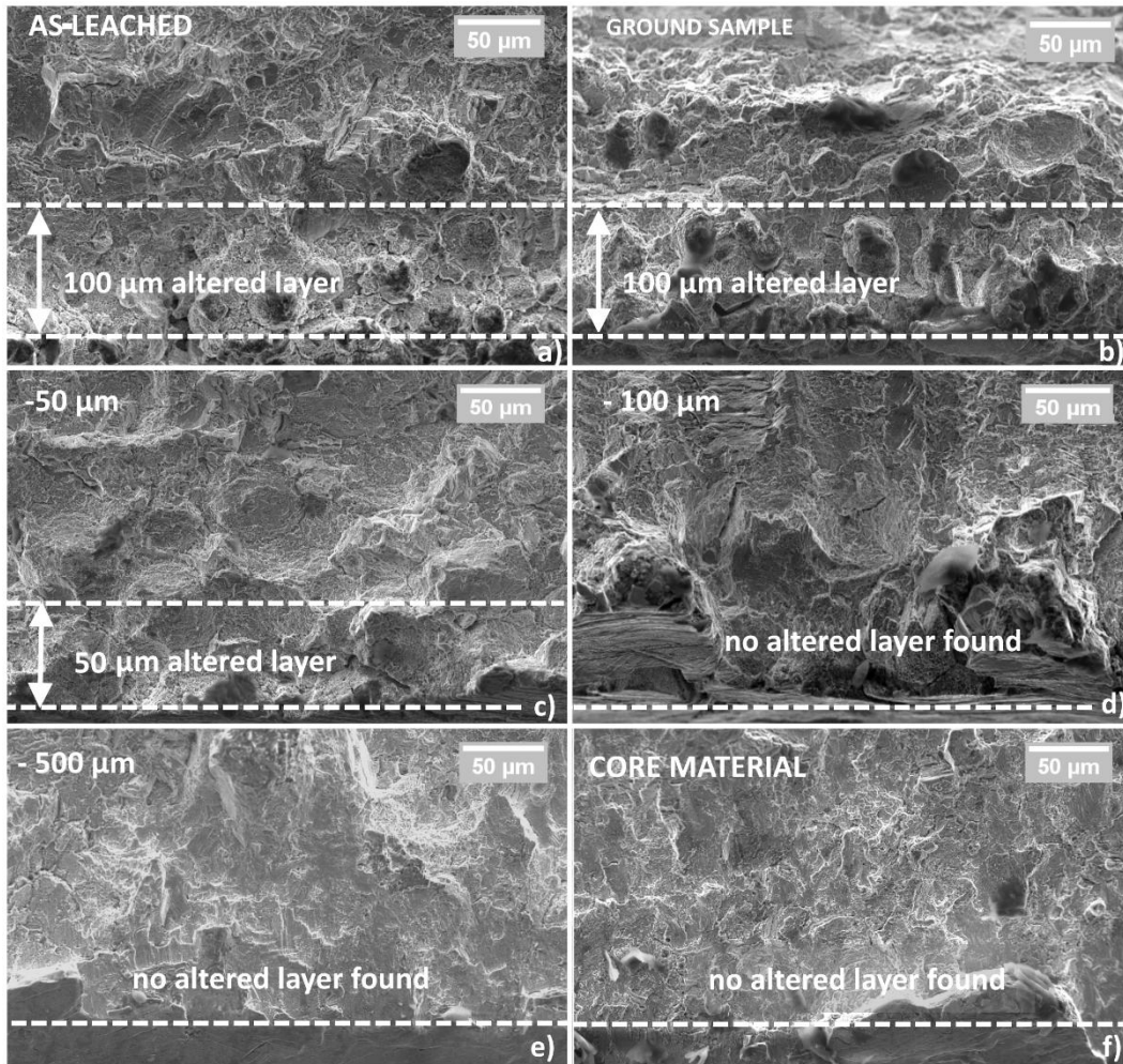
Figure 10 Fractographic surfaces of samples after bending tests taken with secondary electron SEM
