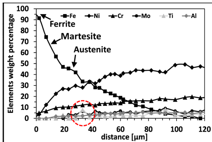
Figure 7: EDS showing compositional gradient located at the interface between Steel capsule and Astroloy surface.
