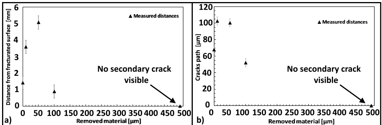
Figure 15 Plot of distance covered by secondary cracks in the samples as a function of removed material
