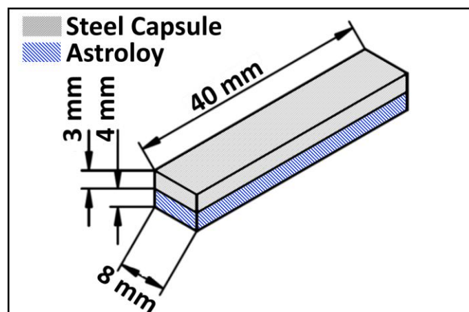
Figure 1 Drawing of the specimen before the acid pickling process
