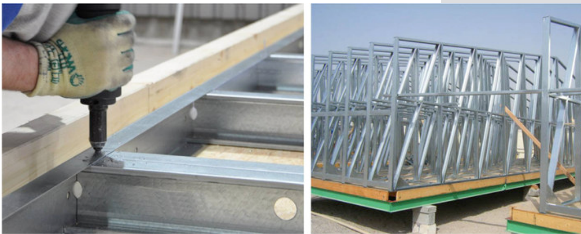
Figure 2. Example of assembly mode to steel frame panel.
