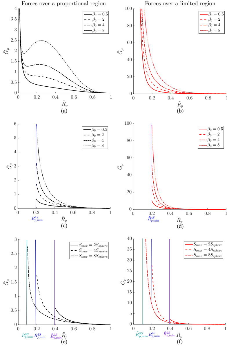
Fig. 3 Critical values of G_\mu below which the cell cannot enter inside a channel of dimensionless radius \tilde{R}_p . The figure reports the plots of \tilde{G}_\mu when the region of contact is the entire cell surface or a fixed proportion of it (and thus it can potentially grow indefinitely) on the left column and when \tilde{L}_b^* is bounded by \tilde{L}_b^M = 5 on the right column. In (a) and (b) \lambda(\Delta S) = \lambda_0 while in (c)-(f) \lambda(\Delta S) = \lambda_0 \Delta S / (S_{max} - S) . In (a)-(d) the value of \beta_0 = \lambda_0 R_n / \mu is changed keeping \mu fixed, whereas in (e)-(f) the value of S_{max} is changed keeping \beta_0 = 2 . We denote with \tilde{R}_{p,min}^{kS} ( k = 2, 4, 8 ), the minimum radius of the channel corresponding to the maximum extension of the nucleus membrane S_{max} , supposed equal to kS_{sphere} .
