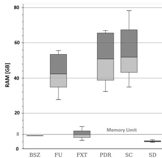
Fig. 6. Memory usage of collapser tools.
