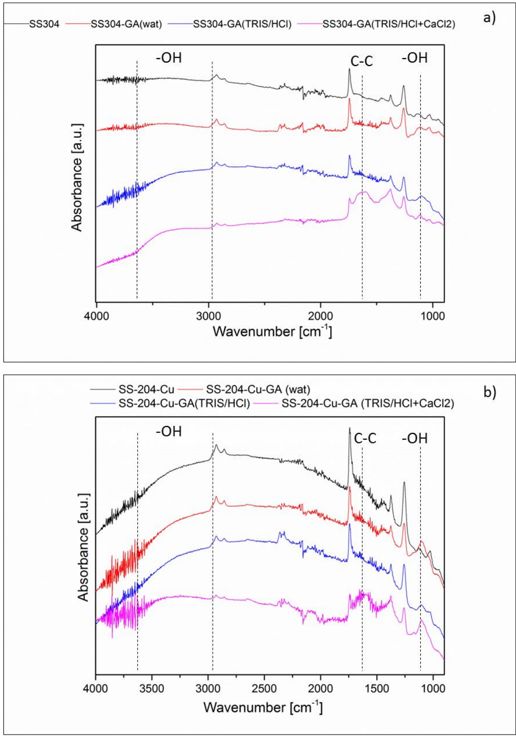
Figure 4: FTIR spectra of the substrates and GA-grafted steel surfaces :(a) SS 304, (b) SS 204-Cu.
