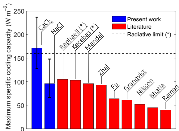
Fig. 4. Comparison with other passive cooling technologies. Comparison between the performance of the proposed device and different daytime radiative cooling technologies from the literature. The results reported refer to the works of Rephaeli et al. (36), Kecebas et al. (37), Mandal et al. (12), Zhai et al. (11), Fu et al. (38), Granqvist and Hjortsberg (16), Nilsson et al. (39), Bhatia et al. (40), and Raman et al. (10). The references labeled with an asterisk refer to modeling results. The maximum specific cooling capacity at a vanishing temperature difference for the proposed device and its uncertainties are estimated from the experimental results by linear fitting (least square method). The thermodynamic limit of daytime radiative cooling is computed at T_A = 30^\circ\text{C} (13).
