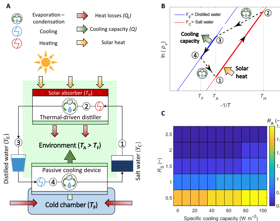
Fig. 5. Stable operating cycle of the passive cooler. (A) Schematic of a possible coupling between the passive cooler and a thermal-driven device for salt water distillation. In the latter device, an external source of heat (e.g., solar) allows water to be distilled from salt water, specifically to regenerate the salinity gradient between the two solutions. Therefore, if the distilled water equals that consumed by the cooler, a stable and passive cooling cycle can be established. The heat dissipation from the top condenser of the cooler and the bottom condenser of the distiller can be ensured by either natural or forced convection. (B) Representation in the Clapeyron chart of a possible coupling between the passive cooler and a thermal-driven device for salt water distillation. For simplicity, the temperatures of evaporators and condensers are equal to those of the surrounding environments ( T_A and T_F , respectively). The salt water contained in the condenser operates ideally at ambient temperature ( T_A ) and constant concentration ( Y_C ) (point 1). The draw solution, diluted by the cooling device, is constantly regenerated by the solar distiller. A selective solar receiver passively heats the salt water (point 2, temperature T_H ), producing distilled water ( Y_E ) at ambient temperature (point 3). This can be used by the proposed device (point 4) to cool a chamber to a temperature lower than the environmental temperature. (C) Coupling between the cooling device and the passive solar distiller proposed by some of the authors (19). R_S is the ratio between the number of stages of the distiller and those of the cooler; R_A is the ratio between the solar collecting area of the distiller and the active area of the cooler. Potential regeneration capabilities of the salinity gradient in the cooler are evaluated considering that the condensers are fed by salt water, with NaCl concentration equal to 170 g liter -1 .
