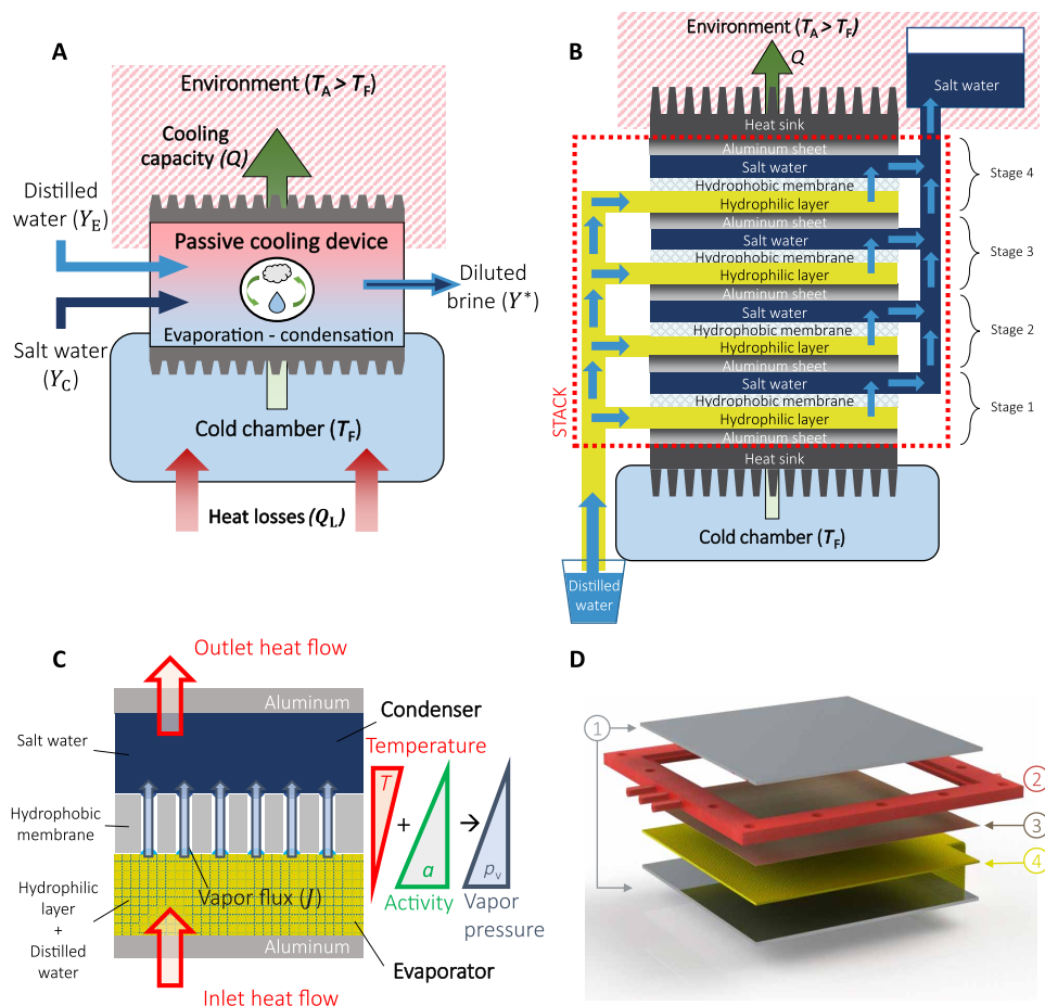
Fig. 1. Layout, schematics, and working principle of the passive cooling device. (A) Schematic of the working principle of a generic salinity-driven cooler: The salinity difference between two inlet solutions generates a net vapor flux from the evaporating ( Y_E ) to the condensing ( Y_C ) layers. These evaporation-condensation processes in multiple stages allow the removal of heat from the lower-temperature chamber and the transfer of heat into the higher-temperature external environment. This process eventually leads to a by-product, being the dilution of the solution in the condensers, which is here represented as an outlet flow with an intermediate salinity ( Y^* ) with respect to the inlet solution at Y_C . (B) Schematic layout of the four-stage modular passive cooler discussed in this work. The actual experimental setup is reported in fig. S1. (C) Working principle of one stage of the passive cooler: Two solutions with different salinities are separated from each other by a hydrophobic membrane. The salt concentration difference creates an activity gradient (green triangle), which leads to a net vapor flux. The transfer of enthalpy of evaporation establishes a temperature gradient between the two solutions (red triangle), which is opposed to the gradient created by the activity difference. (D) Graphical representation of the assembly of one stage of the cooling device. A 3D-printed plastic frame (2, red) contains the cavity that forms the condenser, which is sealed by an aluminum plate cover (1, gray) and a hydrophobic membrane (3, brown). The hydrophilic layer (4, yellow), being the evaporator, is placed between the membrane and another aluminum plate.
