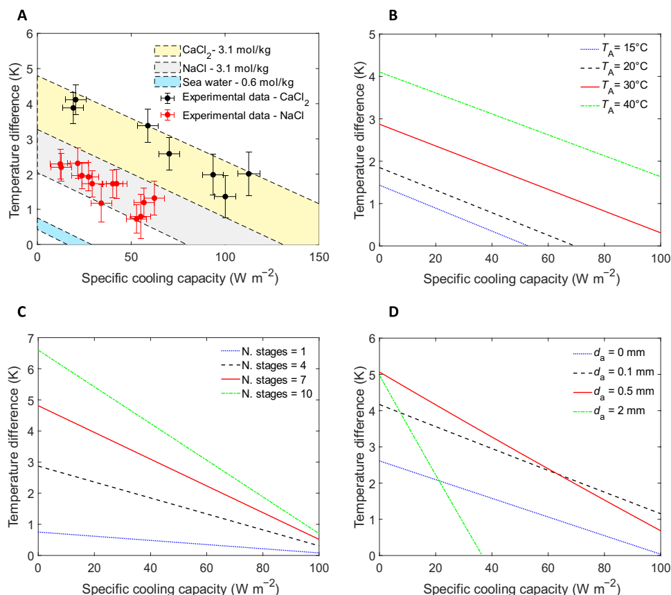
Fig. 3. Cooling performance with different configurations. (A) Cooling performance of the four-stage passive cooler as predicted by the lumped parameter model for different aqueous solutions. While the evaporators contain distilled water in all cases, the condensers are supposed to contain seawater ( 0.6 \text{ mol/kg} , blue band), a 3.1 \text{ mol/kg} solution of NaCl (gray band), or a 3.1 \text{ mol/kg} solution of \text{CaCl}_2 (yellow band). (B) Modeling predictions for the four-stage passive cooler at different ambient temperatures ( T_A ) but a fixed 3.1 \text{ mol/kg} NaCl solution. According to Eq. 4, a higher T_A implies greater vapor fluxes through the membrane, hence better cooling performance than the case that was experimentally assessed (solid red line, T_A = 30^\circ\text{C} ). The increase in cooling capacity with the ambient temperature is mainly due to the exponential increase of vapor pressure with temperature, as predicted by Antoine's law. (C) Modeling predictions for the passive cooler with different numbers of stages but a fixed 3.1 \text{ mol/kg} NaCl solution and T_A = 30^\circ\text{C} . Increasing the number of stages substantially increases the maximum temperature difference achievable across the device owing to the reduction of the temperature across each membrane. (D) Modeling predictions for the four-stage passive cooler considering an additional air gap beneath the membrane, as predicted by the lumped parameter model. In detail, the performance of the cooling device is estimated by varying the thickness of the additional air gap ( d_a ) from 0 to 2 mm, with a 3.1 \text{ mol/kg} NaCl solution and T_A = 30^\circ\text{C} . All the model parameters used in (A) to (D) are reported in table S1.
