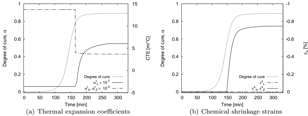
Figure 10: Loads evolution during the curing process.
