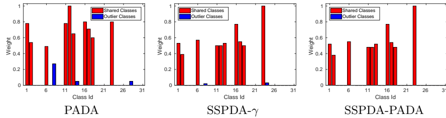
Fig. 2. Histogram showing the elements of the \gamma vector, corresponding to the class weight learned by PADA, SSPDA- \gamma and SSPDA-PADA for the A→W experiment.
