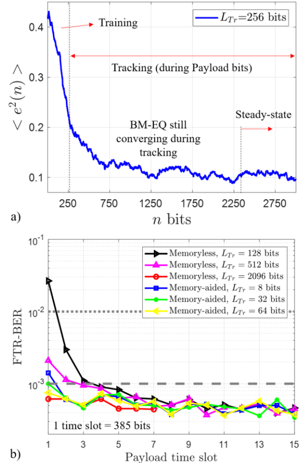
Fig. 10 a) Error square evolution over time for a given L_{Tr} ; b) FTR-BER over each of the 385-bit time slots for memory-aided and memoryless BM-AE approaches with different training length L_{Tr} . ODN loss = 28.7 dB.
