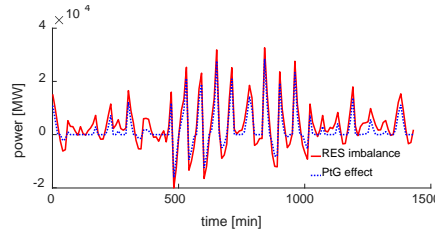
Fig. 8. Load profiles for 2040gca scenario, 1984 climatic conditions (January)
