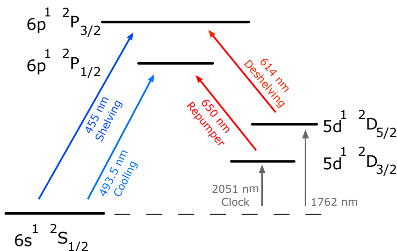
Figure 3.1: ^{138}\text{Ba}^+ ion Grotrian scheme [108].
