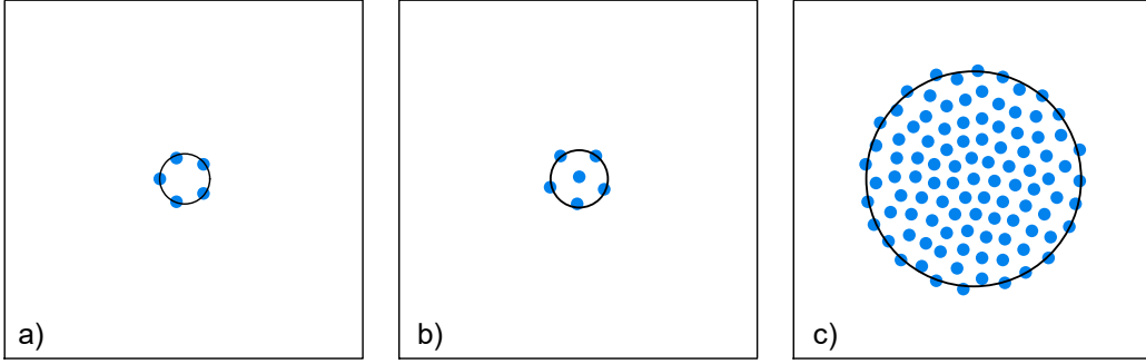
Figure 3.8: Monte Carlo simulations of Coulomb crystals with different numbers of ions: a) 5 ions, b) 6 ions and c) 100 ions. The trap frequency is 2\pi \cdot 1 MHz. The crystals are enclosed by circumferences having radii a) 3.7 \mu\text{m} b) 4 \mu\text{m} and c) 15 \mu\text{m} . The box side is 50 \mu\text{m} long.
