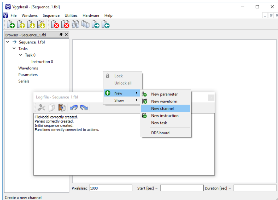
Figure 6.3: Screenshot of a new born file “Sequence_1.fbl”. The docked browser along the floating Log file are shown. The white space behind the log file is the empty ChannelViewer, an Yggdrasil custom view.
