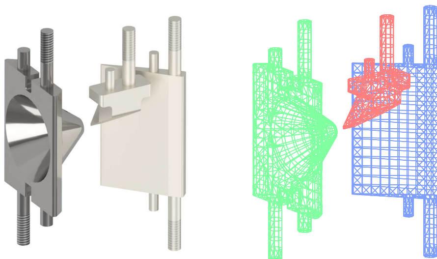
Figure 4.12: On the left, a composition of the three electrode typologies. On the right, their mesh representation.
