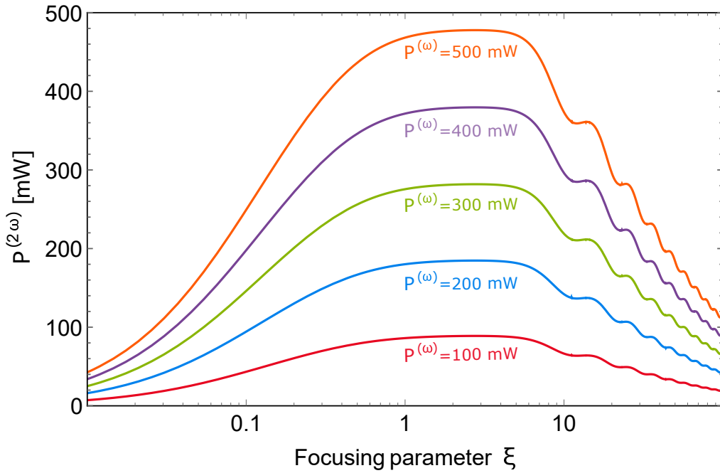
Figure 5.20: SH power plotted for different fundamental powers as a function of the focusing parameter \xi . If \xi = 1 , it means that the pump beam is considered collimated in the crystal.
