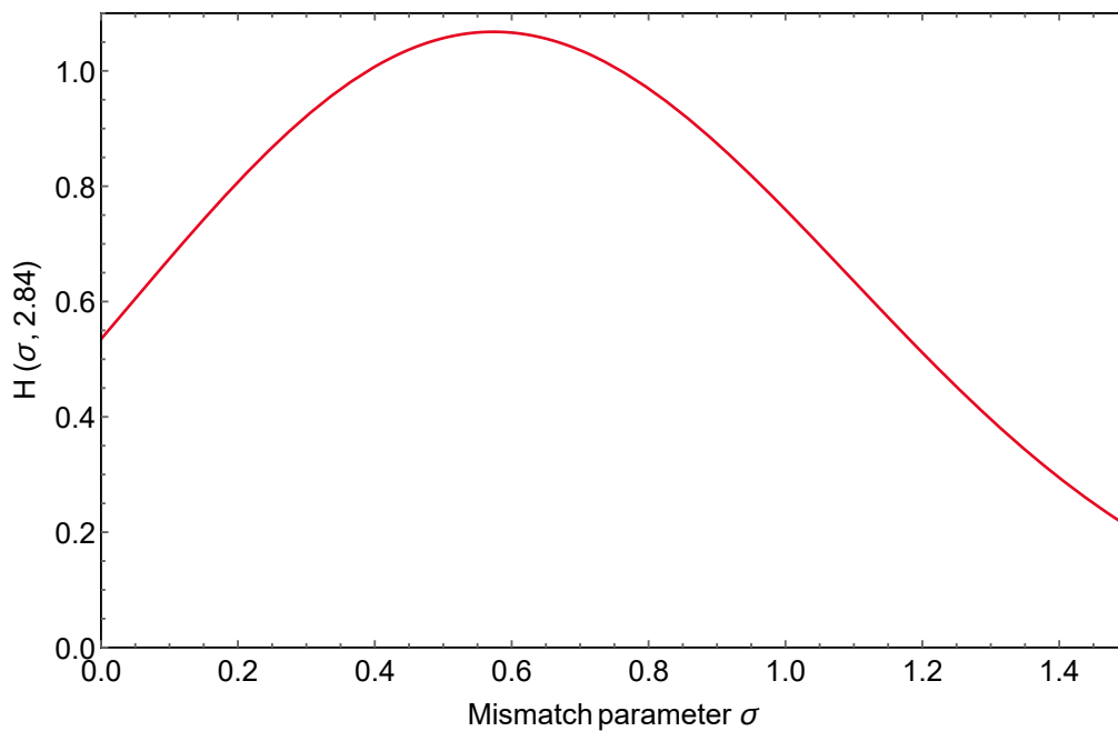
Figure B.2: Plot of the function H(\sigma, \xi) with the optimized focusing parameter \xi = 2.84 . Its maximum value assumed is 1.068.
