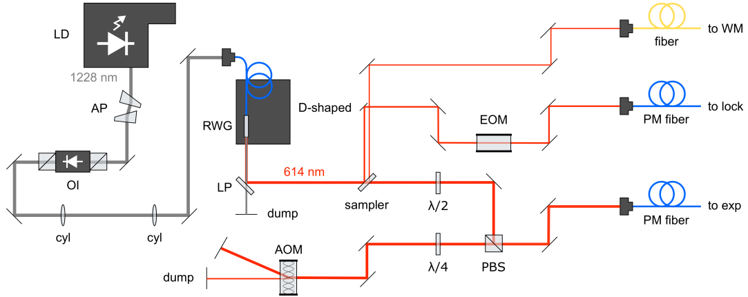
Figure 5.22: Scheme of the deshelving laser production via single-pass second harmonic generation.
