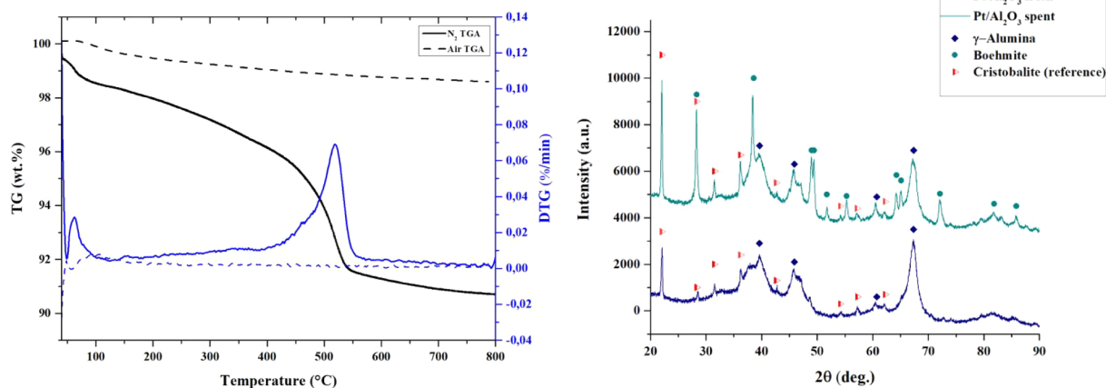
Fig. 14. Thermogravimetric analysis of the spent catalyst performed first in nitrogen and subsequently in air (left) and XRD analysis of the fresh and spent catalyst with cristobalite as internal standard (right).
