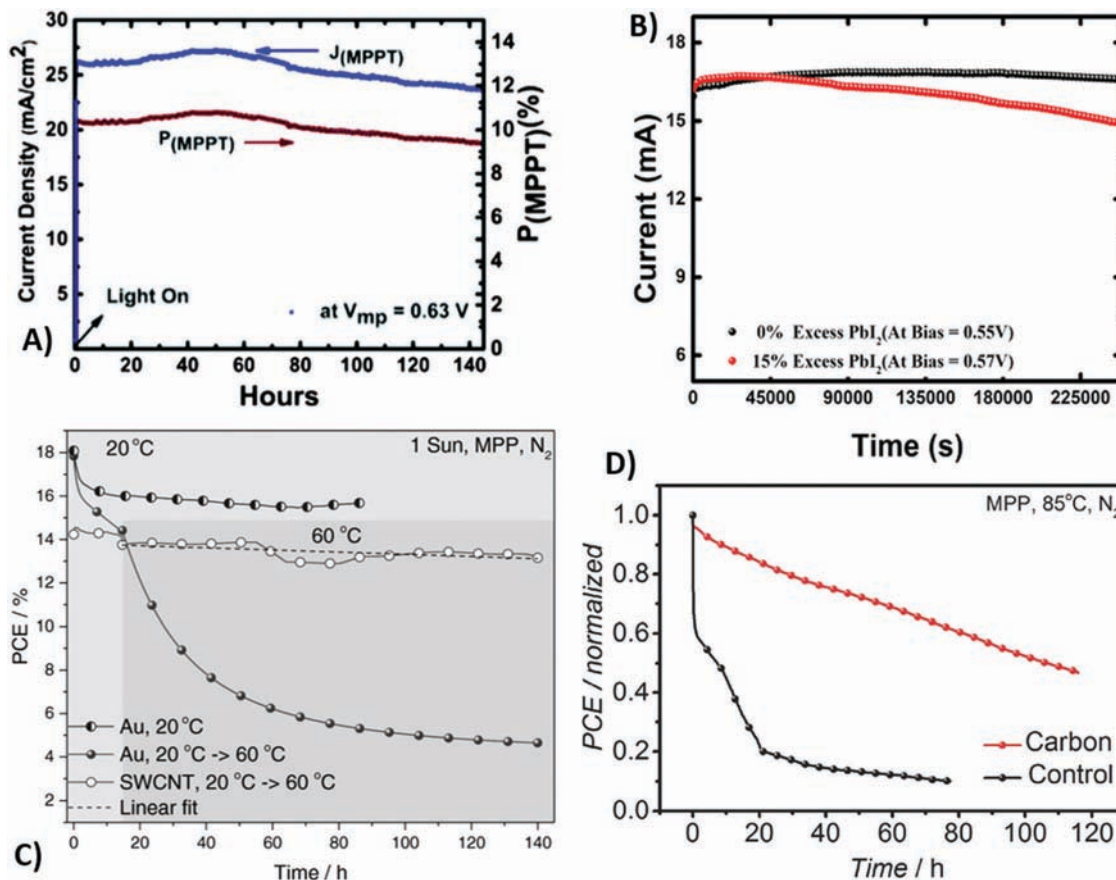
Fig. 18 Aging tests at the MPP under light for: (A) a \text{Co}_3\text{O}_4/\text{carbon} solar cell; (B) carbon-based PSC with or without \text{PbI}_2 excess; (C) gold- and single-walled CNT-contacted devices at elevated temperatures; (D) carbon cloth- and gold-based cells (under a \text{N}_2 atmosphere, 85 °C). Adapted and reprinted with permission from ref. 158, 228, 329 and 330.
