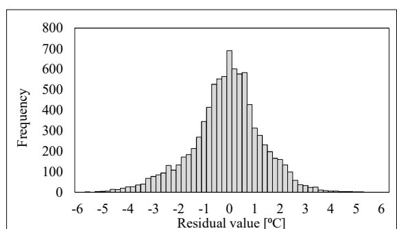
Fig. 12. Histogram of temperature residuals (hourly values).
