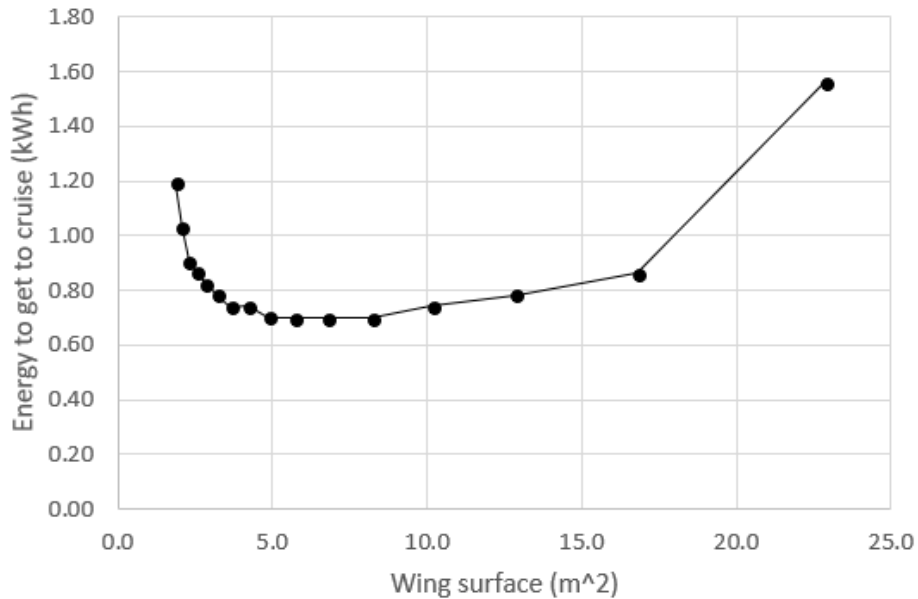
Figure 11: Energy required to get from hover to cruise speed function of the wing surface.
