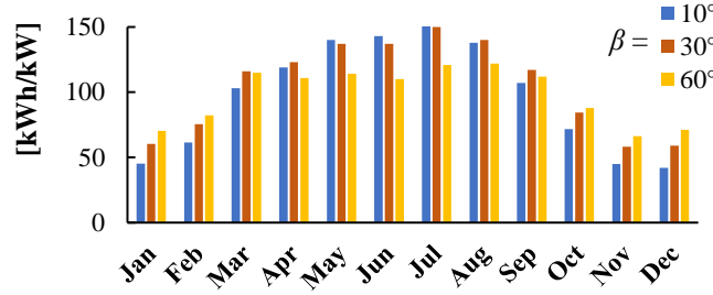
Fig. 1. PV production , with \gamma=26^\circ (SW) and different inclinations \beta .
