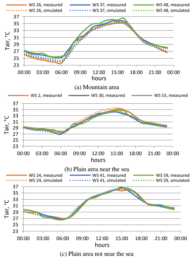
Figure 14. Distribution of the hourly air temperature for August 19 th 2013
