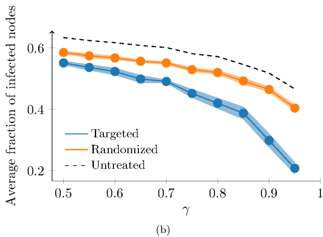
FIG. 7. Monte Carlo estimation over 100 runs of the effect of randomized (orange) and targeted (blue) immunization on the fraction of infected nodes. Dotted lines indicate the fraction of infected nodes in the absence of any immunization technique. In (a), we show the entire realizations for \gamma = 0.95 . The solid line is the average, while the light band is one standard deviation. In (b), we compare the average fraction of infected nodes for different values of \gamma . Bands identify 95% confidence intervals. Other parameters are n = 300 , \beta_d = \beta_a = -3 , \lambda = 0.9 , and \mu = 0.1 .
