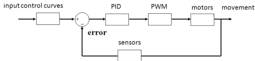
Figure 8. P.I.G.R.O. control structure for each lower limb joint.
