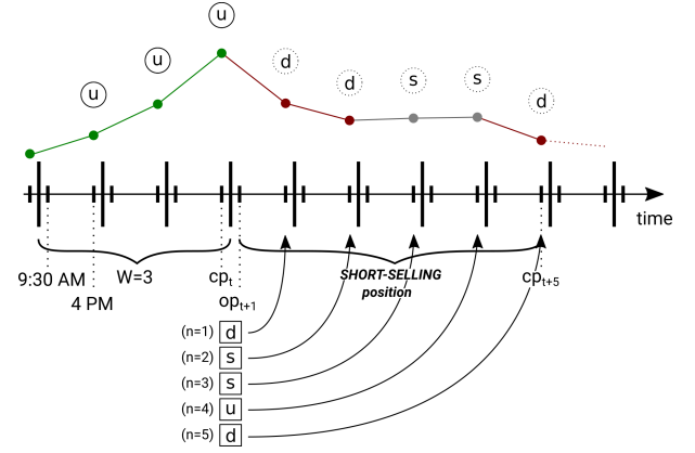
Fig. 1. Trend detection and reversal prediction.
