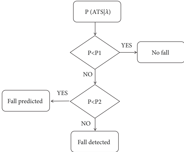
FIGURE 4: Threshold-based algorithm.
