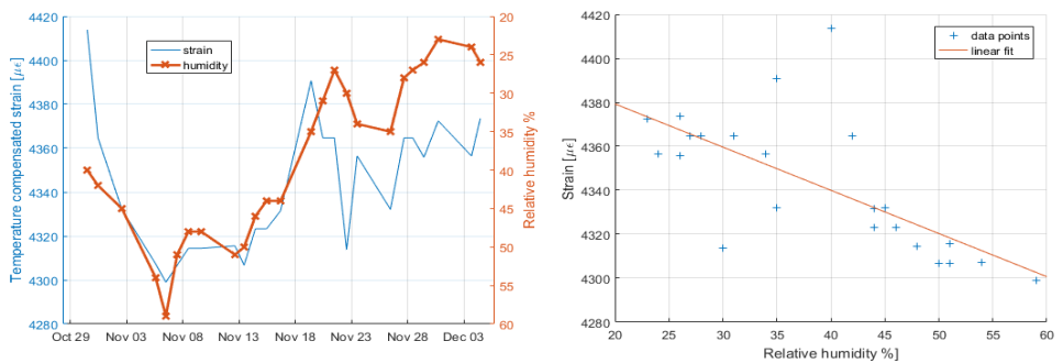
Fig. 6. Temperature compensated strain and humidity (left); linear fit of strain vs humidity (right); example for the Epoxy Resin sample.
