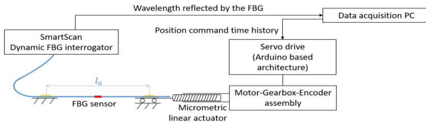
Fig. 3. Setup of the second experiment.
