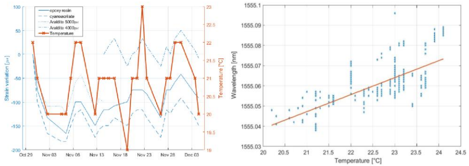
Fig. 5. Variation of measured strain and room temperature versus time (left); Linear fit of wavelength versus room temperature (right).
