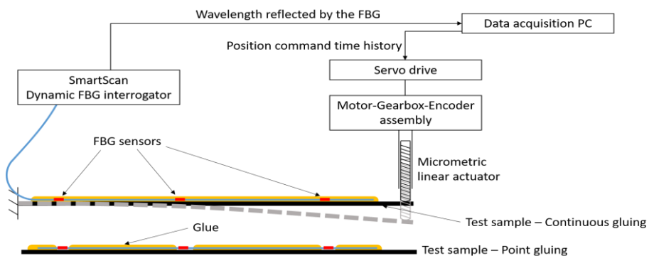
Fig. 1. Setup of the first experiment.
