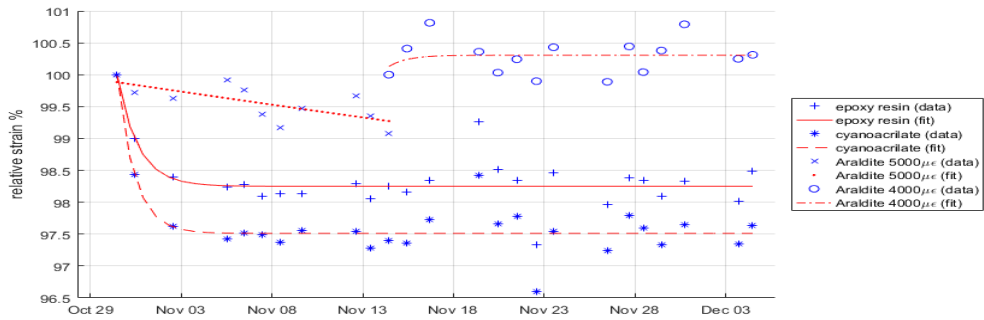
Fig. 7. Relative compensated strain (as a fraction of initial value) and exponential fit. Note that the two Araldite samples have too few data points for an effective fitting
