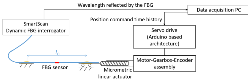
Fig. 3. Setup of the second experiment.
