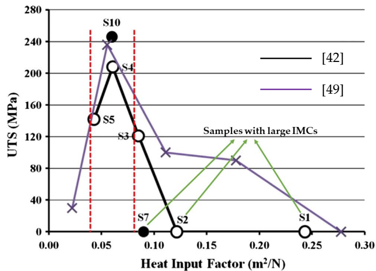
Figure 9. Relationship between joint strength and heat input factor in FSW of AA5186 and mild steel (Reproduced from [42], with permission from Elsevier, 2013).
