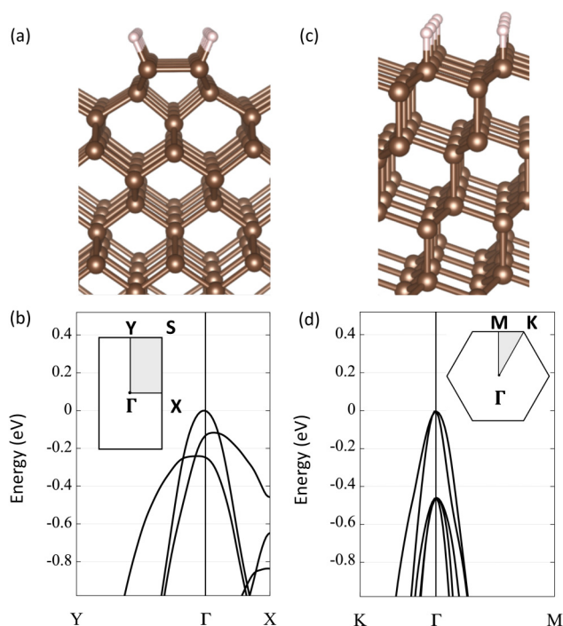
FIG. 1. (a) Ball-and-stick model of the hydrogen-terminated, reconstructed (100) 2 \times 1 diamond surface, and (b) the relevant electronic bandstructure. (c), (d) Same as (a), (b) for the hydrogen-terminated, unreconstructed (111) 1 \times 1 diamond surface. Large brown spheres and small pink spheres are carbon and hydrogen atoms, respectively. The zero of the energy is set to the valence-band maximum. The insets to (b) and (d) represent the first Brillouin zone. Grey shaded areas are the irreducible Brillouin zones. Data in (b), (d) are adapted from Ref. 56.
