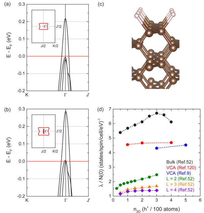
FIG. 7. (a) Electronic bandstructure of the iongated, hydrogen-terminated (110) 1 \times 1 diamond surface for n_{2D} = 2.84 \cdot 10^{13} \text{ cm}^{-2} . The inset shows the first Brillouin zone and the Fermi surface. (b) Same as in (a) but for n_{2D} = 5.68 \cdot 10^{13} \text{ cm}^{-2} . (c) Ball-and-stick model of the crystal lattice. Large brown spheres and small pink spheres are carbon and hydrogen atoms, respectively. (d) Electron-phonon coupling constant normalized to the DOS at the Fermi level, \lambda/N(0) , as a function of n_{2D} in units of induced carriers per 100 atoms. Data in (a), (b) are adapted from Ref. 51; note that only the uppermost valence bands are shown. Data in (d) are adapted from Refs. 9, 52, and 120.
