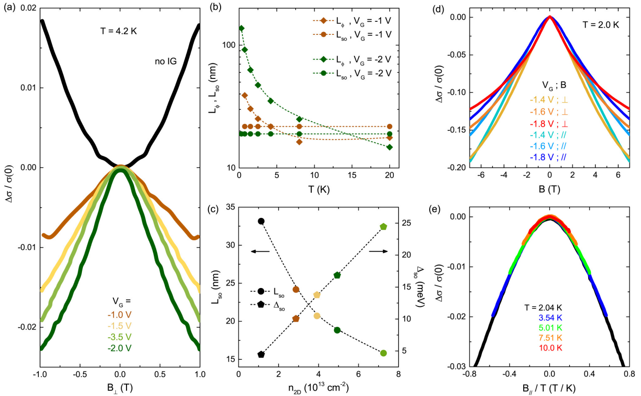
FIG. 5. (a) In-plane magnetoconductance ratio [\sigma(B) - \sigma(0)]/\sigma(0) vs. out-of-plane magnetic field B_{\perp} , for different values of V_G applied at a (100) diamond surface. The label “no IG” marks the curve in absence of the ionic gate. (b) T -dependences of the phase-coherence length L_{\phi} (diamonds) and spin-coherence length L_{so} (circles) for two different values of V_G . (c) Spin-coherence length L_{so} (circles, left scale) and spin-orbit splitting \Delta_{so} (pentagons, right scale) as a function of n_{2D} . Dashed lines in both (b) and (c) are guides to the eye. (d) In-plane magnetoconductance ratio [\sigma(B) - \sigma(0)]/\sigma(0) as a function of either the out-of-plane magnetic field B_{\perp} (orange-red lines) or the in-plane magnetic field B_{\parallel} (green-blue lines) for different values of V_G . (e) In-plane magnetoconductance ratio vs. B_{\parallel}/T . Data for different values of V_G = -1.4, -1.5, -1.8 V and T (as indicated in the legend) all collapse on the same curve. Data in (a), (b) and (c) are adapted from Ref. 47. Data in (d) and (e) are adapted from Ref. 48.
